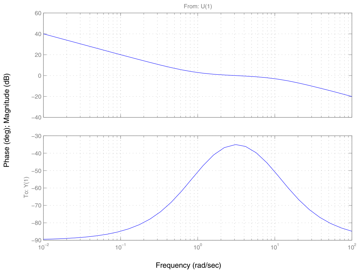
Bode Diagrams
